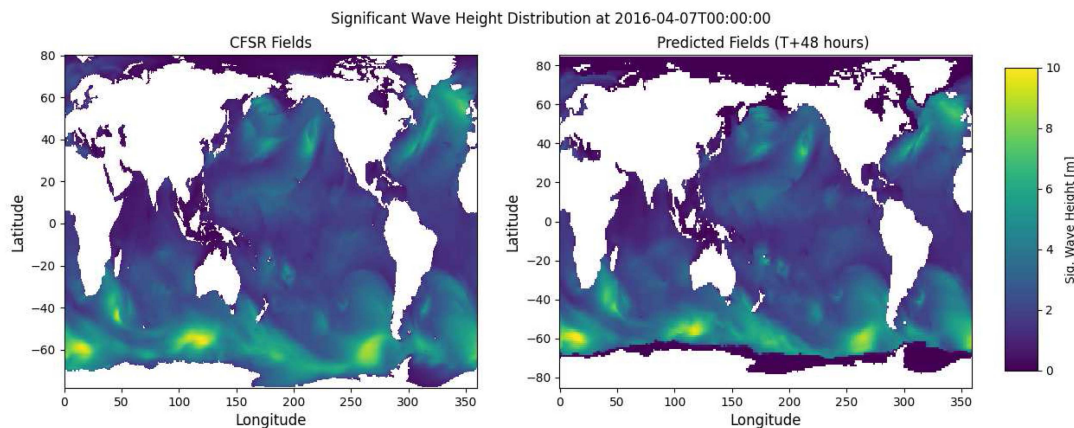
Fig. 3. Comparison between wavefields obtained from the CFSR hindcasts (left) and the forecasts (right) obtained using the WWIII model without the forcing applied for the forecast horizon.
