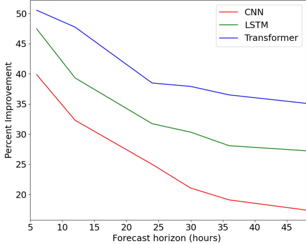
Fig. 5. Percentage improvements of CNN, LSTM, and Transformer for different forecast horizons using WaveWatch III hindcasts.
